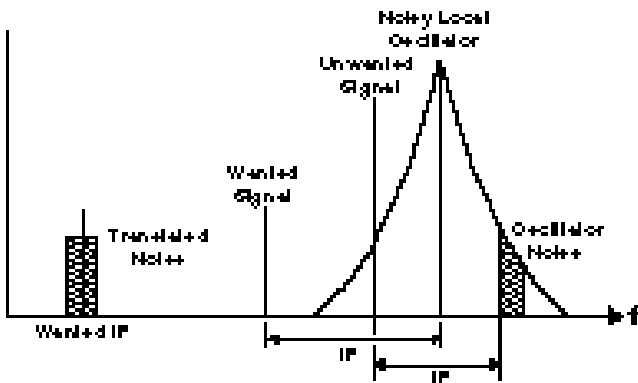
Fig. 15 Reciprocal mixing
